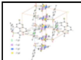
Fig. 2. \pi\cdots\pi , C—H \cdots\pi and C—H \cdots O interactions (dotted lines) in the title compound. Cg denotes the ring centroids. [Symmetry codes: (i) x-1/2, -y+3/2, z-1/2 ; (ii) -x+1, -y+1, -z+1 ; (iii) -x+1, -y+2, -z+1 ; (iv) x, y+1, z ; (v) x, y-1, z ; (vi) x+1/2, -y+3/2, z+1/2 .]
